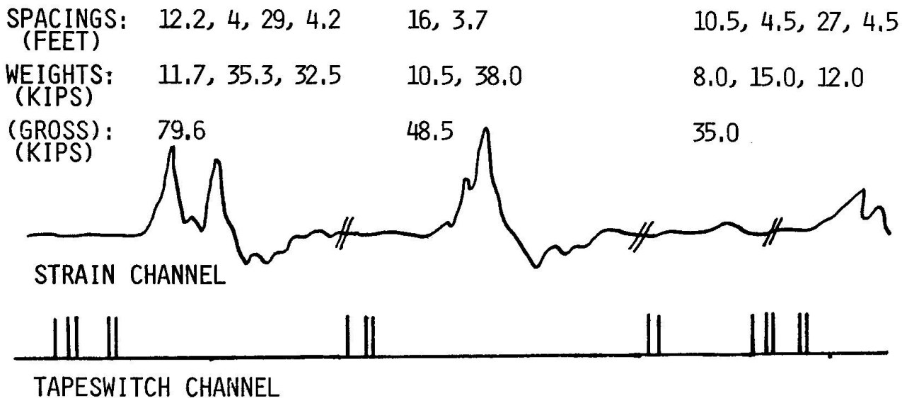
FIGURE 2 SAMPLE RECORD FROM WIM SYSTEM SHOWING BRIDGE STRAIN OUTPUT, TAPESWITCH SIGNALS AND AUTOMATICALLY PROCESSED TRUCK AXLE AND GROSS WEIGHTS, DIMENSIONS AND SPEEDS [4].
