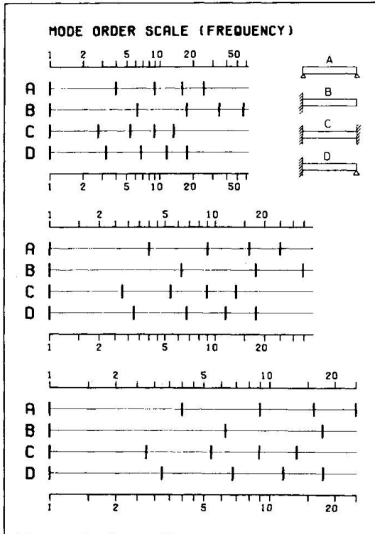
Fig.13 Frequency scales.
