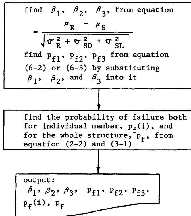
Fig. 5 Flow Chart of the Program for Calculation of the Probability of failure
