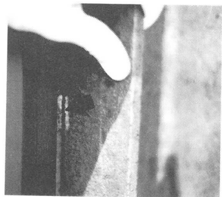
WRONG: Unprotected Faying Surfaces Result in Broken Welds.
