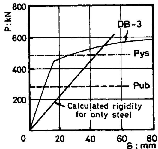
Fig.16 Load-deflection curves of DB-3
