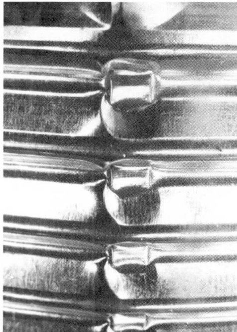
Fig. 6 Support Crippling
