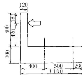
Fig.11 Loading setup
