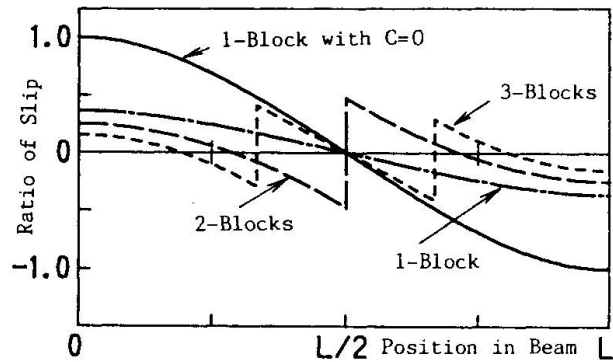
Fig.6 Axial Slip of Slab ( C=100MN/m/m )
