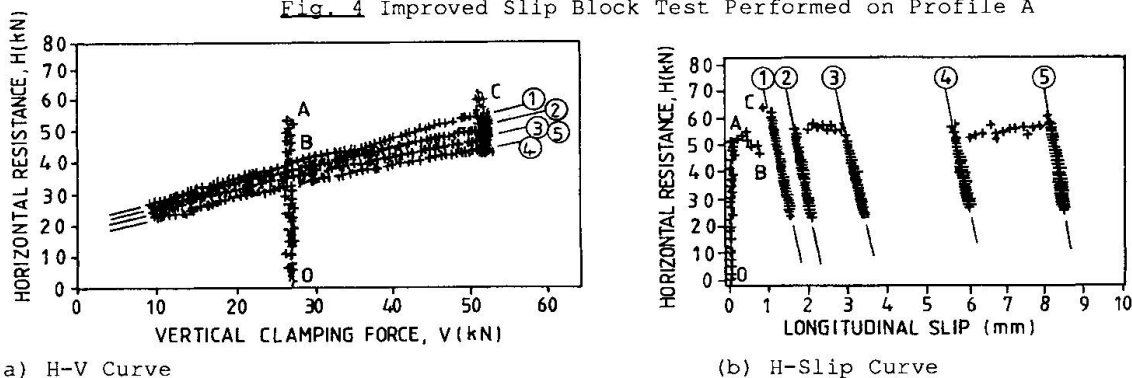
(a) H-V Curve
