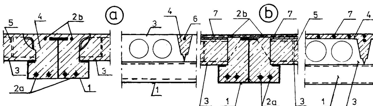
Fig.2. Supporting of precast panels on the steel girder a - normal panel + monolithizing concreting b - prestressed panel + in-situ concrete
