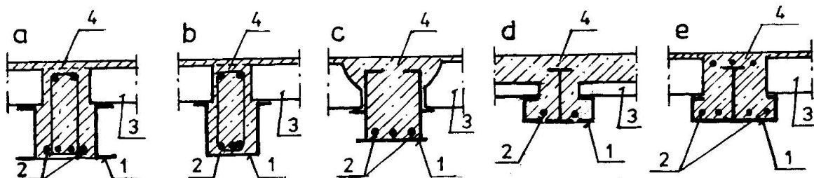
Fig.1. Steel girder composite by concrete slab :
