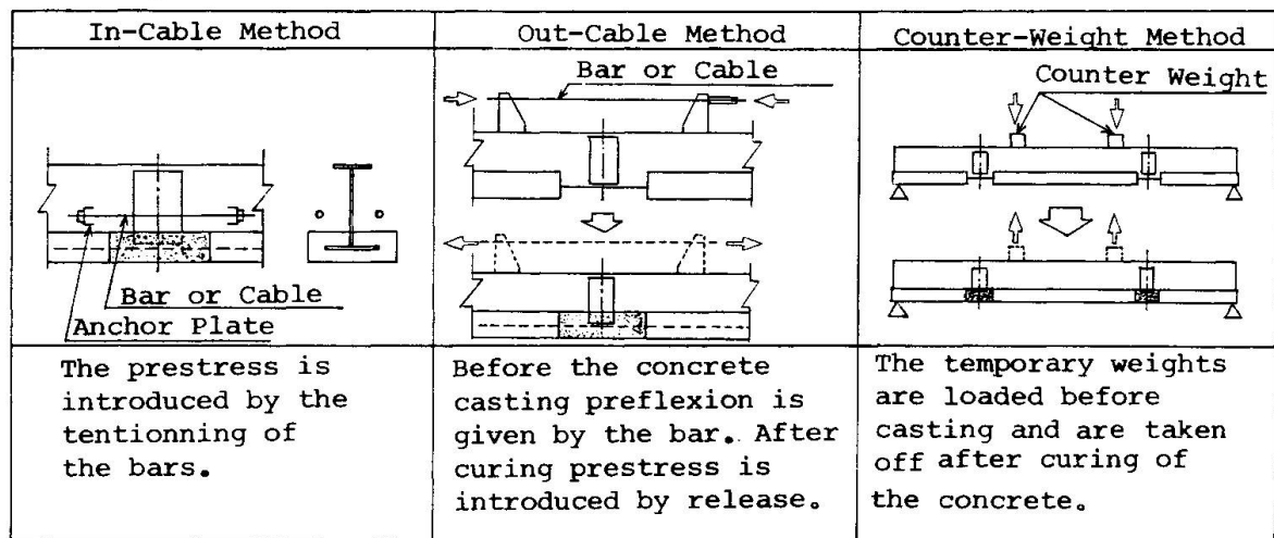
Fig.2 Prestressing Method for Post-Casting Lower Flange Concrete
