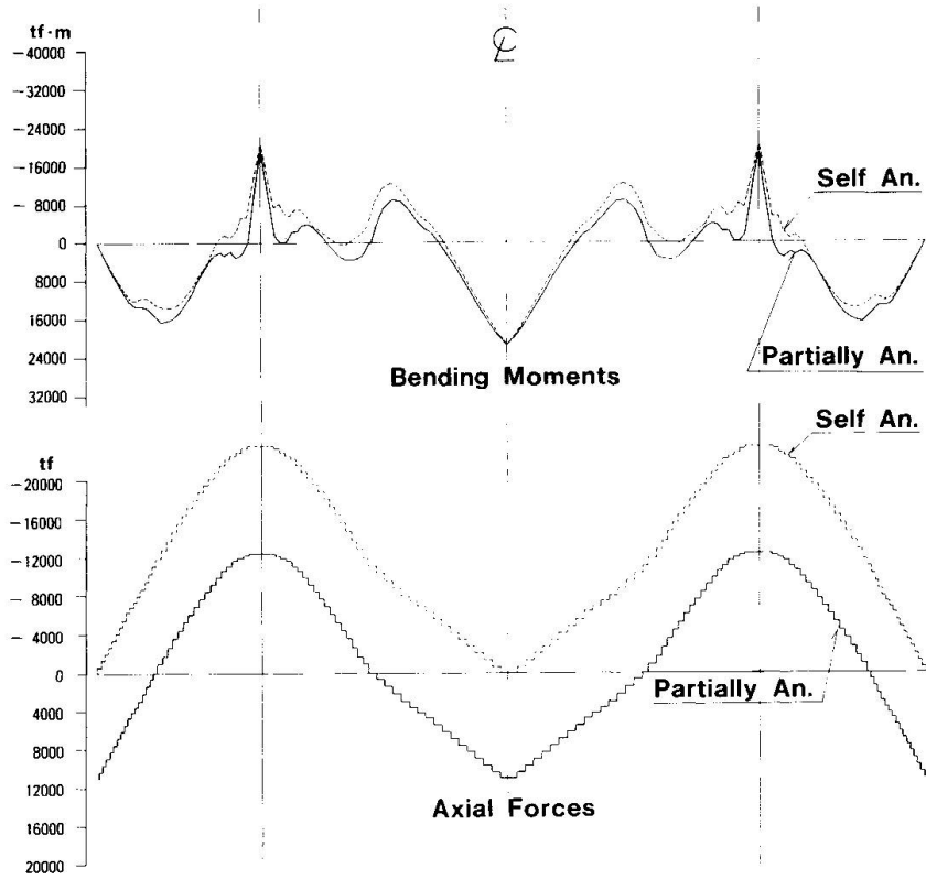
Fig.4 Bending Moments and Axial Forces (1 tf \cdot m = 9.81 \text{ kN} \cdot m )
