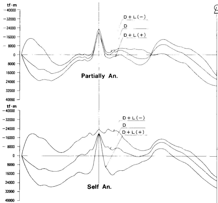
Fig.5 Variations of Bending Moments (1 tf \cdot m = 9.81 \text{ kN} \cdot m )
