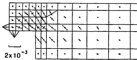
(c) Principal Concrete Strains
