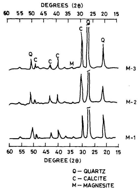
FIG. 4. X-RAY DIFFRACTION (XRD)
