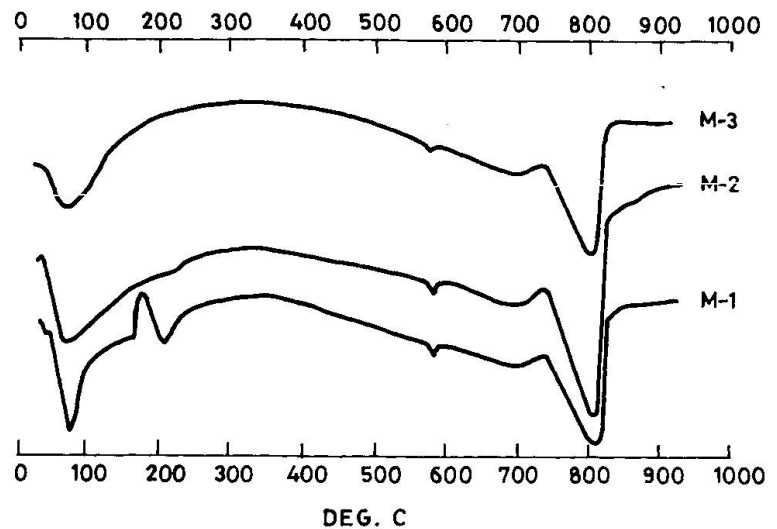
FIG. 3. DIFFERENTIAL THERMAL ANALYSIS CURVES
