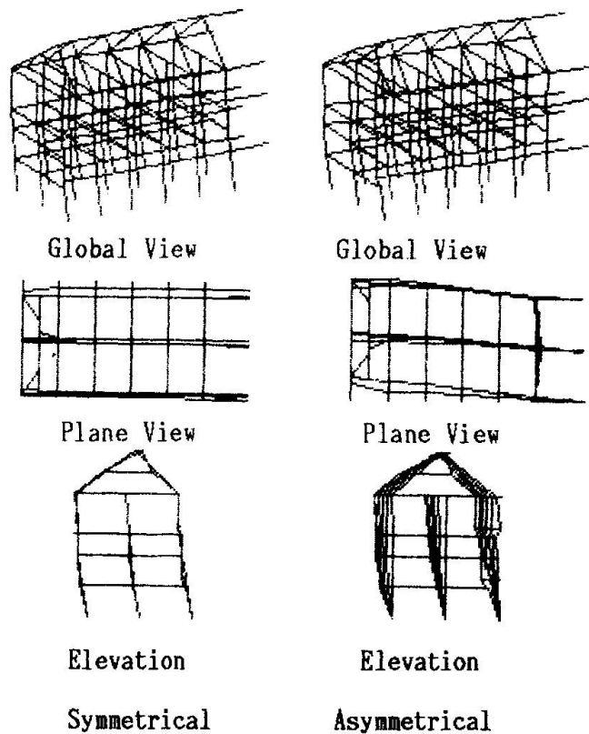
Fig.11 1st Vibration Mode Shape
