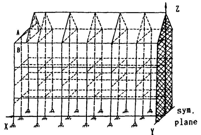
Fig.8 The FEM Model of the Front Tower
