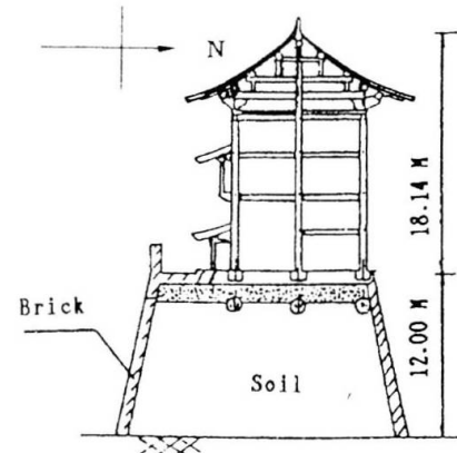
Fig.3 The Elevation
