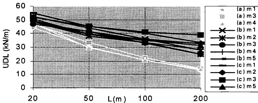
Maximum of the total load (a) flowing traffic, (b) congested traffic with cars, (c) congested traffic without car m1 = half-normal distribution, m2 = Monte-Carlo simulation, m3 = analytical Poisson, m4 = simulation + extrapolation by m3, m5 = jam simulation.
