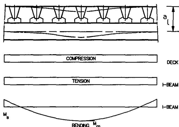
Fig. 9 Model of floating deck crossbeam
