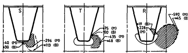
Fig. 12 Stress distributions under vertical load in combination with out of plane bending ( N/mm^2 )
