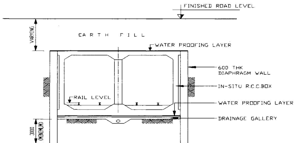
Fig. 3 : Cross Section of Metro : Non-Station Portion (Semi-Integrated Approach)
