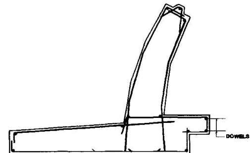
Fig. 7 : R C Details of Unit - 2
