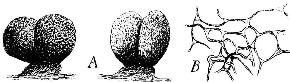
FIG. 2. — Wilczekia Evelinae Meyl.
