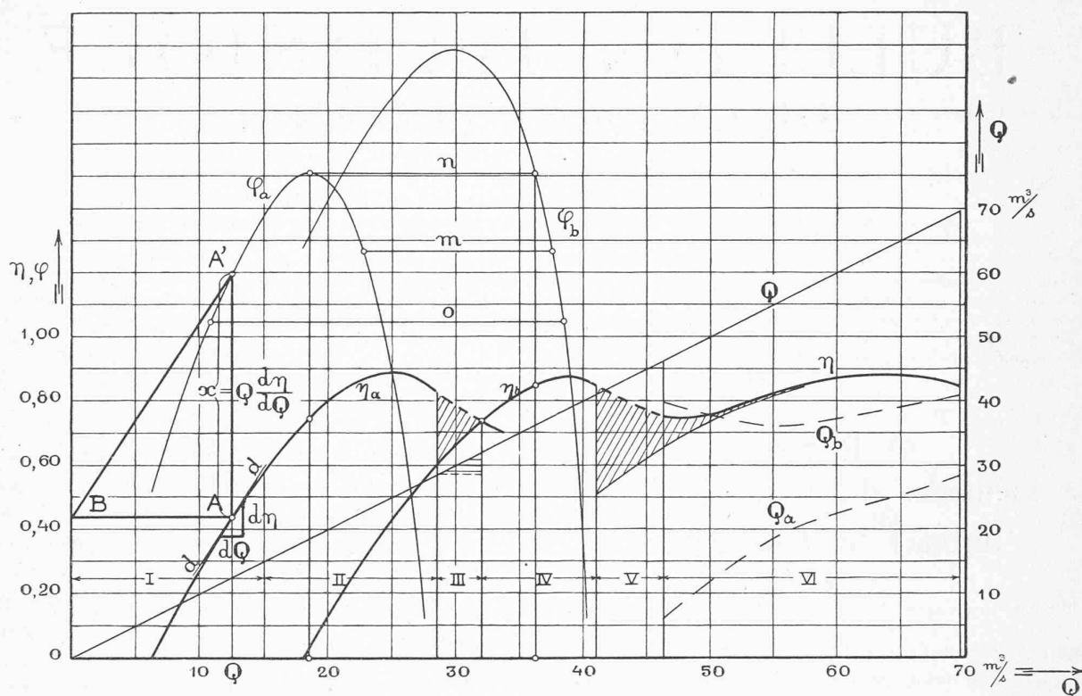
Fig. 1. — Turbine (a) : turbine-hélice ; n_s = 600 ; Q_{max.} = 28,5 \text{ m}^3/\text{sec.}
