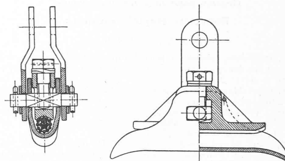
Fig. 2. — Pince de suspension.
