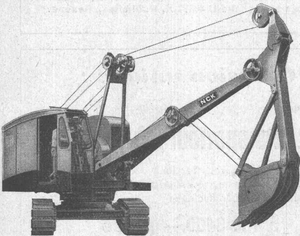
Equipment rétro-caveur
