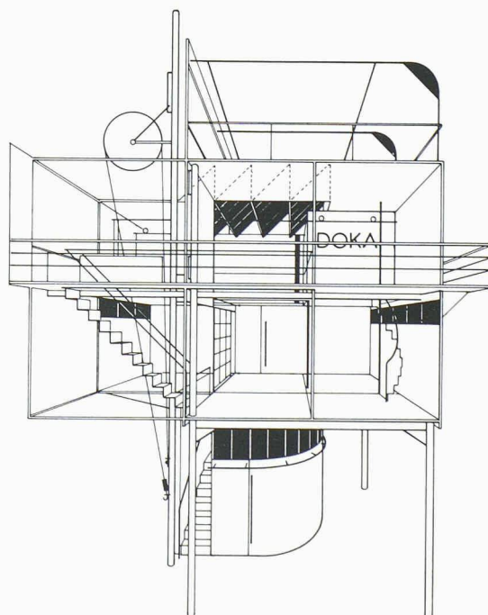
Perspective frontale
