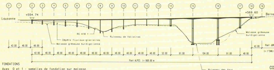
ELEVATION PONT ALPES
