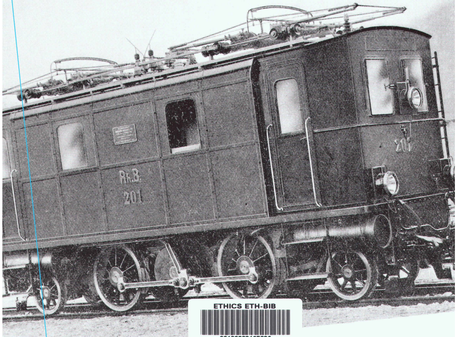
Fig. 9 – Locomotive 1-B-1.
