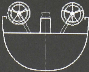
SECTION AT WHEELS 15.115m
