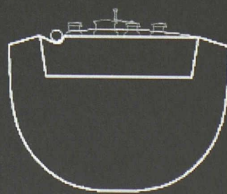
SECTION AT KEEL FRAME 10.343m
