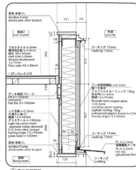
② 床口詳細図 slab connection detail S:1/10
