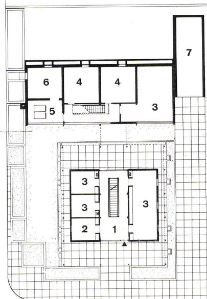
A Grundriß Erdgeschoß / Plan rez-de-chaussée / Plan ground floor 1:400
