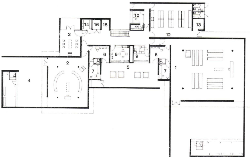
3 Grundriß Kellergeschoß 1:500. Plan de cave. Plan of basement.
