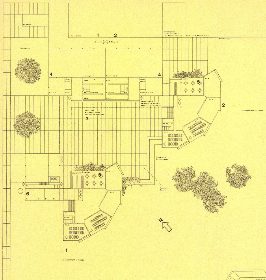
1 Grundriß Erdgeschoß 1:750.
