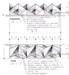
ARTIFICIAL REEF COMPONENT NO. 3 FOLDED HARDWARE CLOTH CONSTRUCTION NOTE: CONTROL REEF (C) IS IDENTICAL EXCEPT FOR ANDING AND ANODIC / CATHODIC CABLES WOODFRAME: 2" x 4" FIF NAILED, MESH FASTENED WITH NAILS
