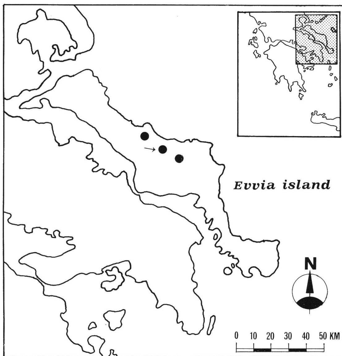
Fig. 3. — Geographical localization of Viola dirphyia . The arrow indicates the type locality.
