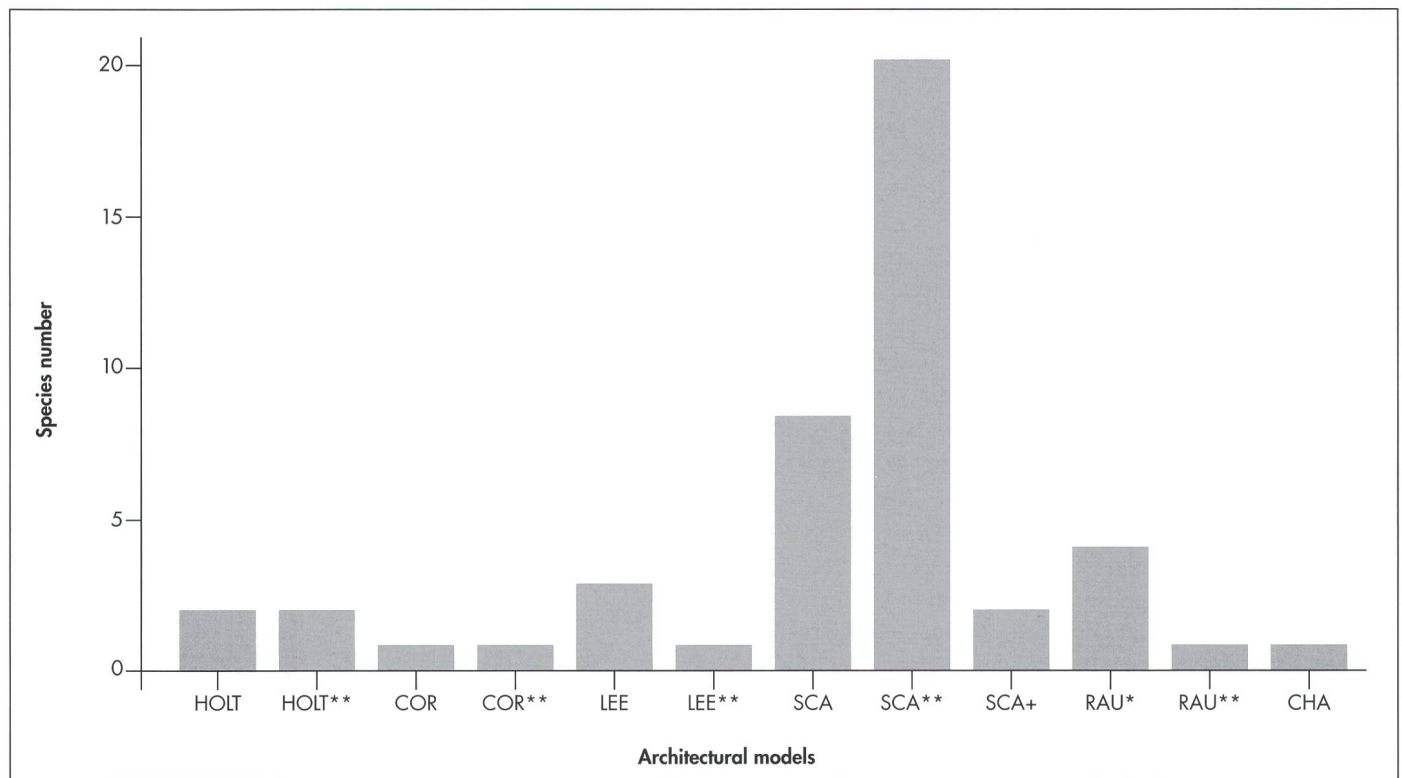
Fig. 2. – Frequency distribution of architectural models of 45 shrub species from Cabo de Gata Natural Park (SE Spain). SCA: Scarrone; RAU: Rauh; HOLT: Holtum; COR: Corner; LEE: Leeuwenberg; CHA: Champagnat. (***) Species conforming to the variant with basitonic repetition of the Holtum, Corner, Leeuwenberg and Rauh models. (*) Species conforming to the sympodic variant of the Rauh model with mixed axes. (***) Species conforming to the sympodic variant of the Scarrone model, but may conform to the Leeuwenberg model in sunnier sites. (+) Species conforming to the sympodic variant of the Scarrone model.
