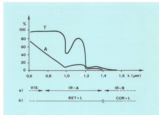
Fig. 3 Transmission and absorption in the eye T Transmission A Absorption a) Subdivision of wavelength bands VIS Visible light IR-A Infrared, zone A IR-B Infrared, zone B b) Possible eye injury RET Retina L Lens COR Cornea
