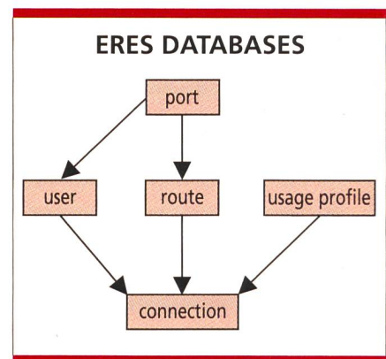
Fig. 1. The five main eReS data bases and its relationships.
