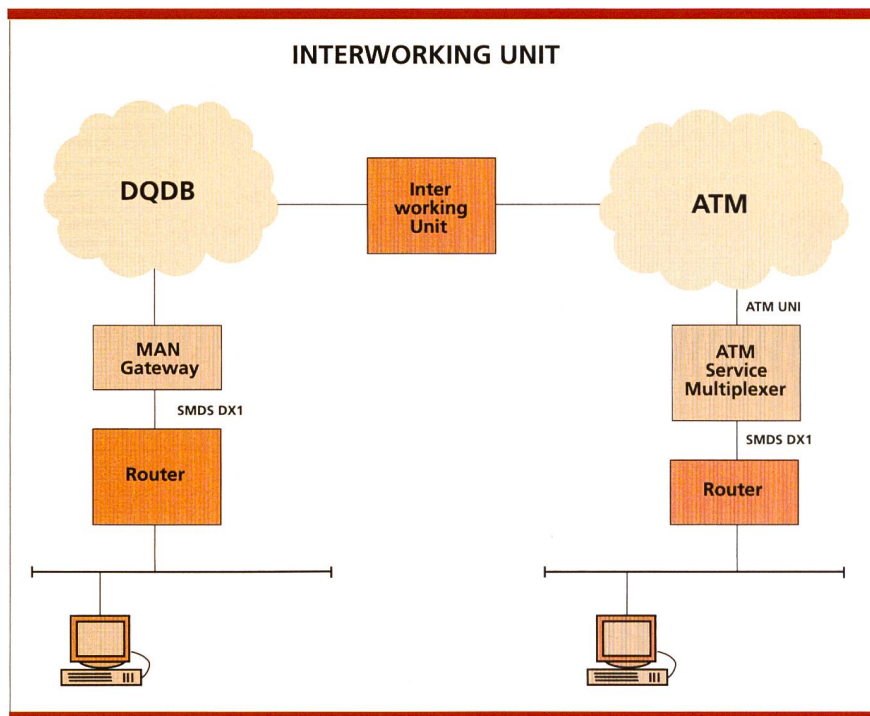
Fig. 3. Interworking unit.
