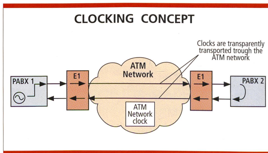
Fig. 1. Plesiochronous clocking concept with master-slave PABXs.
