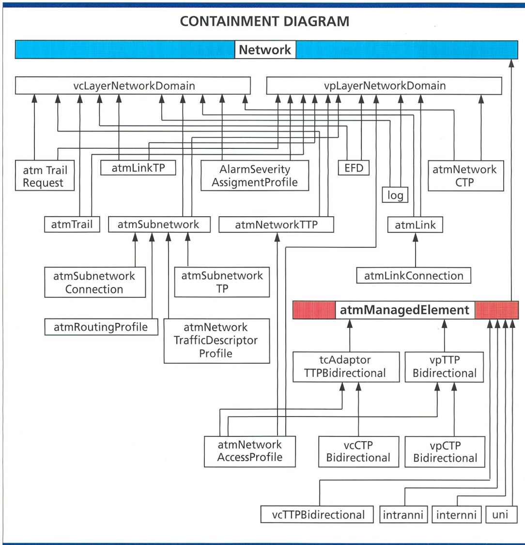
Bild 8a. ATMF M4 Network View: Containment Diagram.
