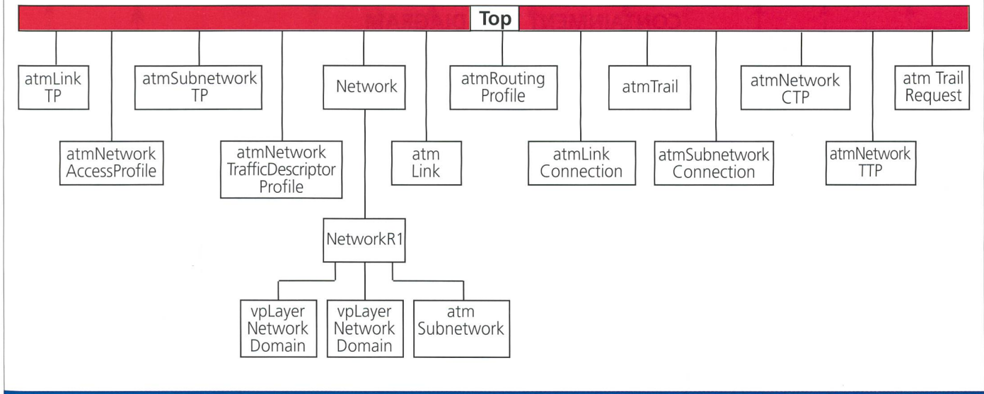
Bild 8b. ATM F4 Network View: Inheritance Diagram.
