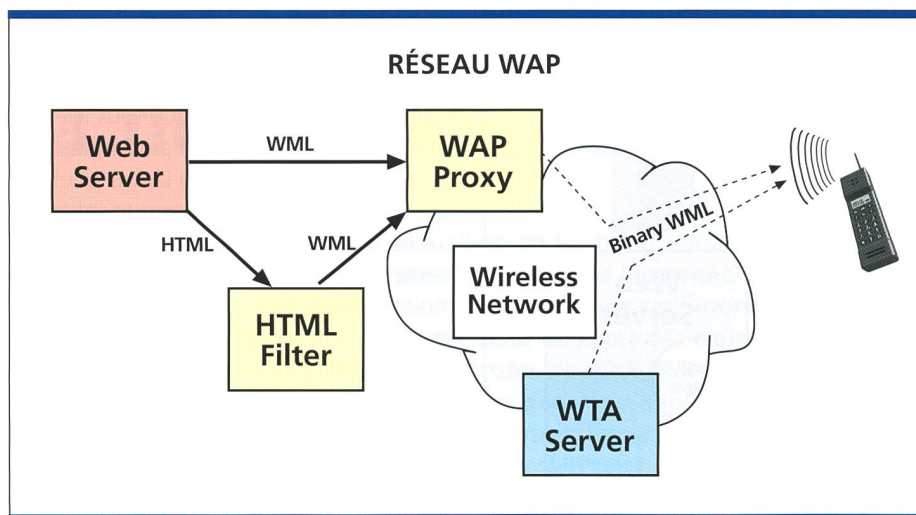
Fig. 3. Exemple de réseau WAP. WAP: Wireless Application Protocol; HTML: Hyper-Text Markup Language; WML: Wireless Markup Language; WTA: Wireless Telephony Application.
