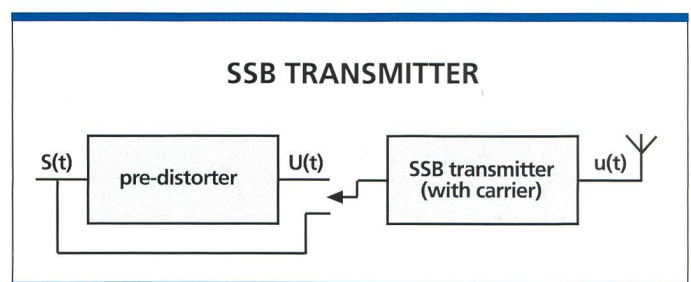
Fig. 1. SSB transmitter with pre-distorter.
