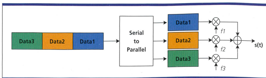
Fig. 1. Simplified view of the process to generate an OFDM signal with 3 subcarriers at frequencies f_1 , f_2 and f_3 .
