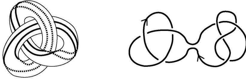
Figure 3. Operations to generate zero-entropy knots: (left) cabling; (right) connected sum.
