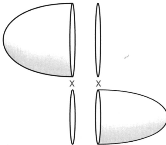
Figure 1. A switched S^3 isometrically embedded in \mathbb{R}^5 .
