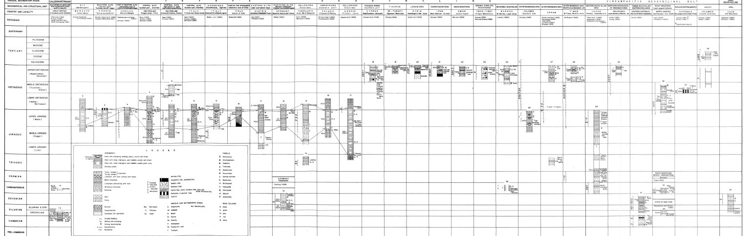
Stratigraphic and geographic distribution of selected radiolarian chert-ophiolite sections. — Not to scale
