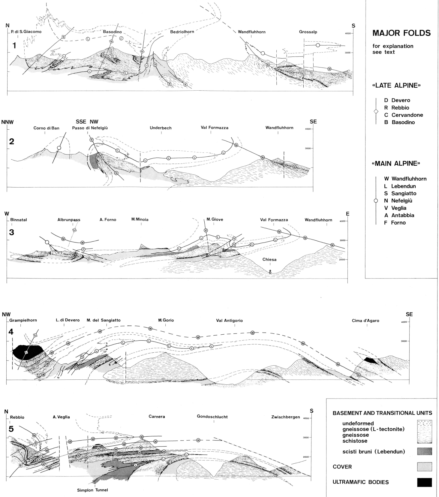
Simplified structural cross-sections of the western Lepontine Alps (for lines of section, see Plate I)
