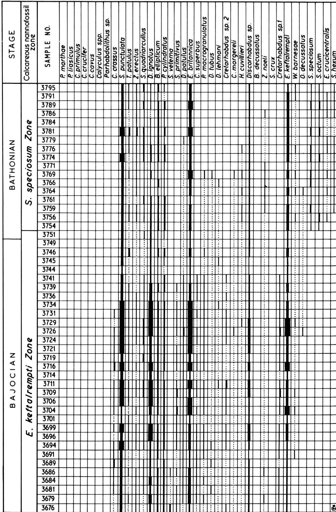
Fig. 5b. The stratigraphic distribution and abundance of calcareous nannofossils in the Bajocian-Bathonian interval of the Brenha Road Section.
