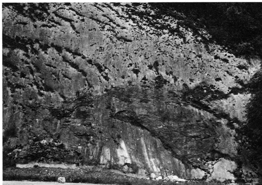
Fig. 13. South limb of Bueberg fold, Lower Oxfordian coral limestones, Birs valley at Bärschwil Station. The somewhat poorly developed bedding planes are supplemented by communicating shear planes. A lower shear plane is characterized by calcite lining and conspicuous striations; it is partly covered by lenticular masses dragged along by upper beds and drawn out and fragmented by tension gashes in the process – a phenomenon similar to that shown in its initial stages in Figures 11 and 12, but much farther developed. Compare also LAUBSCHER (1976, Fig. 17), which is from the left center of the picture.
