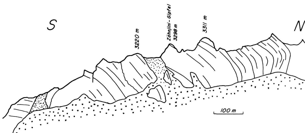
Fig. 8. Large F_2 fold in the Arolla gneisses as seen parallel to the fold axis, looking west from grid ref. 619.4/96.6.
