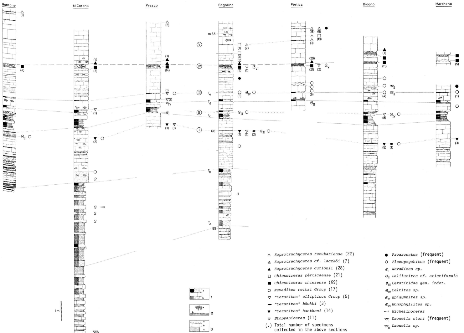
Fig. 7. Correlation and fossil content of selected sections of the lower Buchenstein Beds in the Brescian Prealps and Giudicarie (for location see Fig. 1). The actual distance between the Roncone and Marcheno columns is about 50 km; see text for a short description and location of the columns. 1a = volcanoclastic layers; 1b = mixed siliciclastic and volcanoclastic material; 2a = concentrations of chert nodules; 2b = strongly silicified shales; 3a = beige illite layers; 3b = undulating to nodular limestone beds; 3c = shales.
