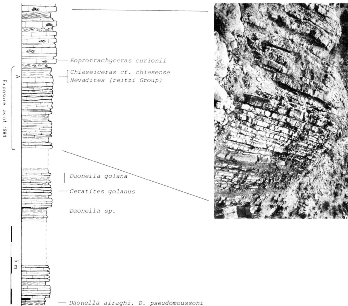
Fig. 8. Exposure of the strata close to the Anisian/Ladinian boundary along the riverbed in Val Gola (near Trento) as it appeared in 1966 and 1984.
