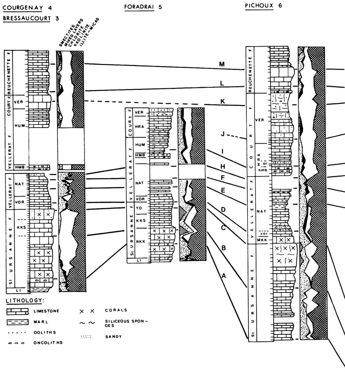
Fig. 9. Lithologic sections with clay mineral distribution, from the carbonate platforms in canton Jura to the deeper marine realm in canton Aargau. The section "Aargau" is assembled of sections no 9 through 11 in Plate 1. Names of formations and members are by THALMANN (1966, p. 32), GYGI (1969, p. 104), and BOLLIGER & BURRI (1970, p. 70).
